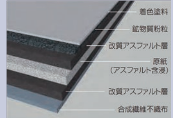
[構成図]
